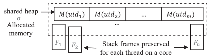
Fig. 3: Memory model
